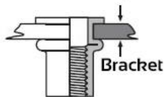
Visual Representation Of When Well Nut When Screw Tightened
