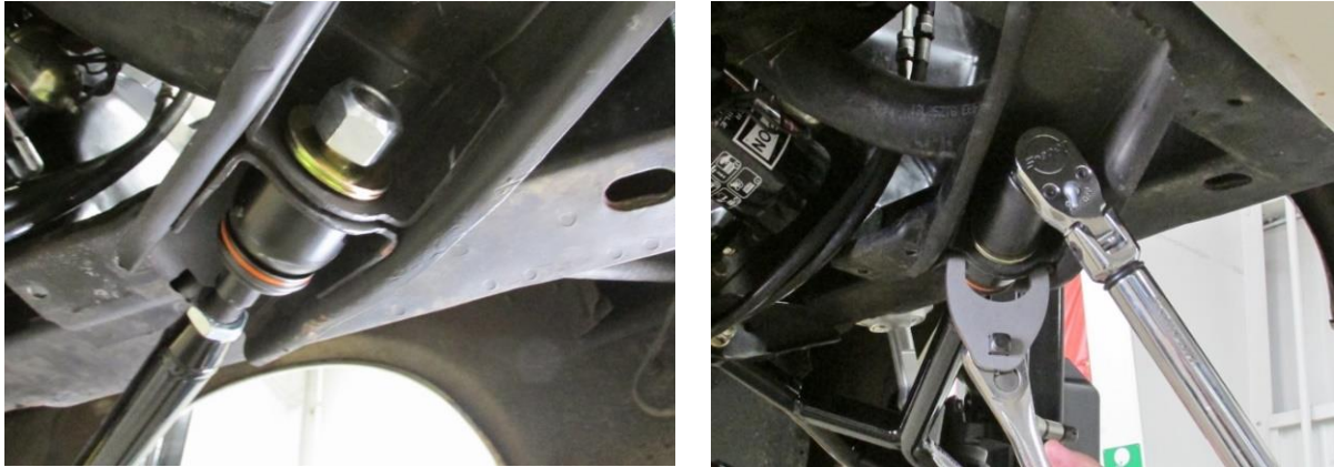
Figure 20 – Install Strut Rod Hardware
