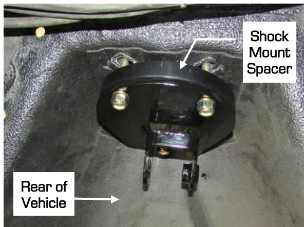
Figure 10 - Install Upper Shock Mounts
